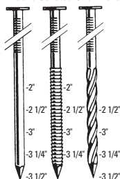
SMOOTH RING SCREW
